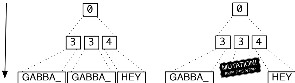
Figure 2: Regular and mutated data generation runs using the CFG inferred in Figure 1
