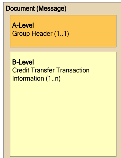
Figure 2: Basic message structure for XML message "pacs.008"
