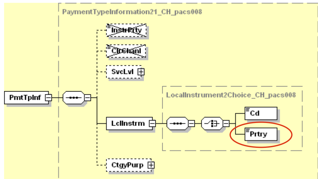
Figure 3: Indication of the payment type in the XML message
