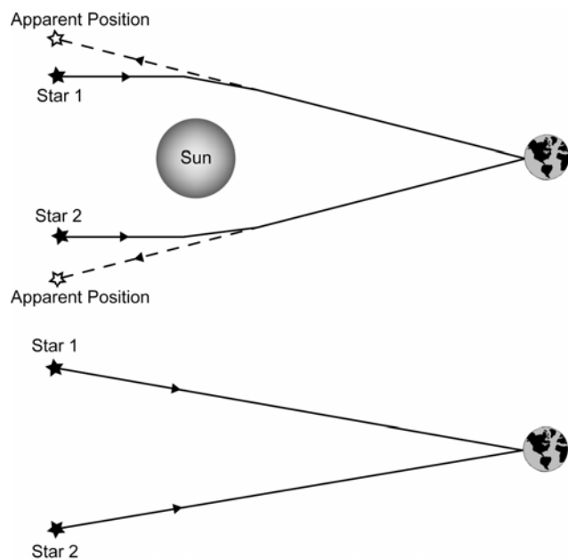
Figure 1.7: The Moon is not shown eclipsing the Sun in the drawings, but this was the case, and necessarily so in order to enable these early 20 th century scientists to see the stars near the Sun during daylight hours. The bottom drawing shows that the angle measured between star 1 and 2 (at nighttime) would be less months later with the Sun out of the that part of the sky. The difference in angle between the stars results from the bending of starlight as illustrated in the top drawing.
