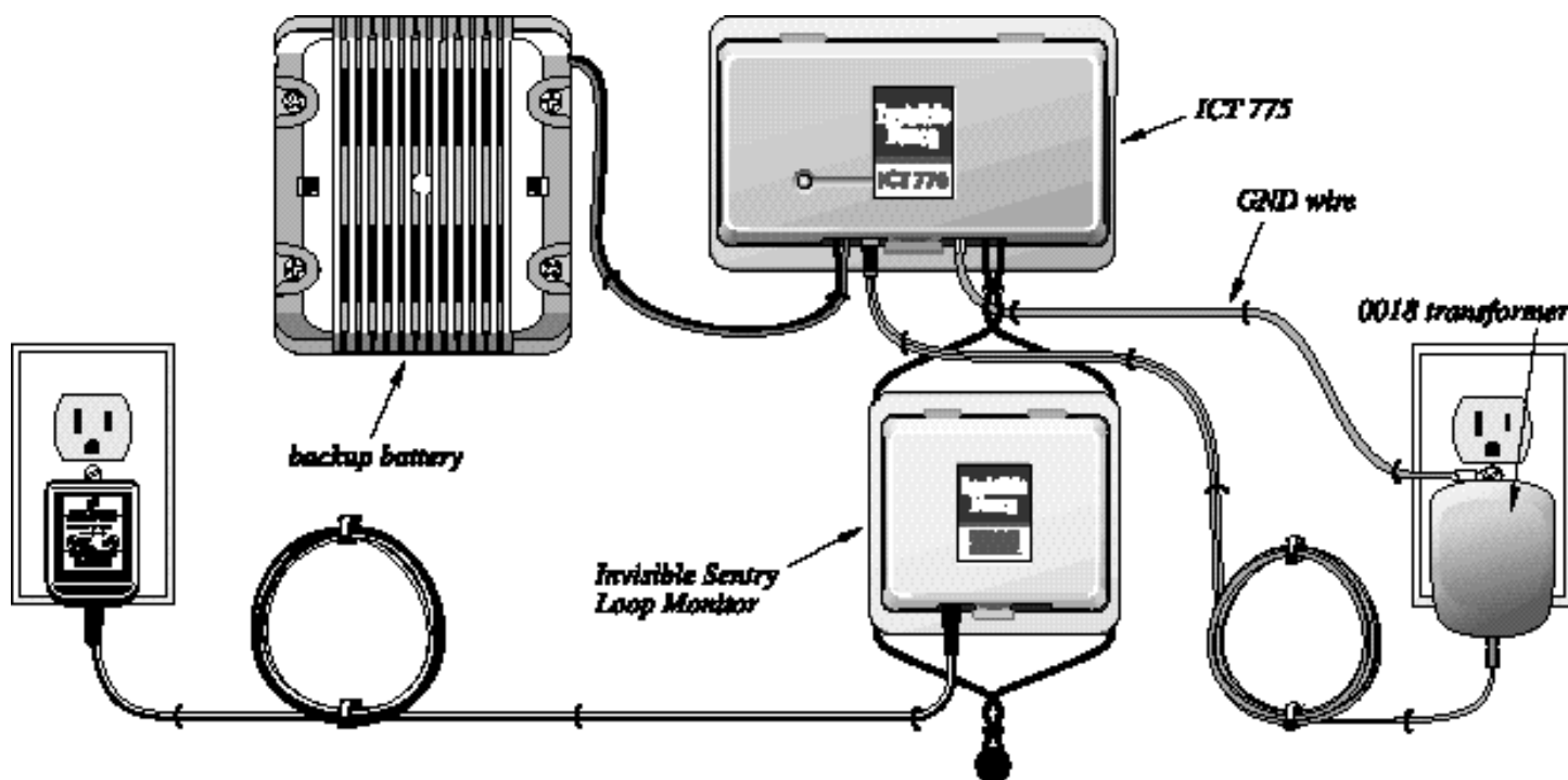
ICT 775 system with a backup battery and an Invisible Sentry™ system monitoring the signal field wire.
