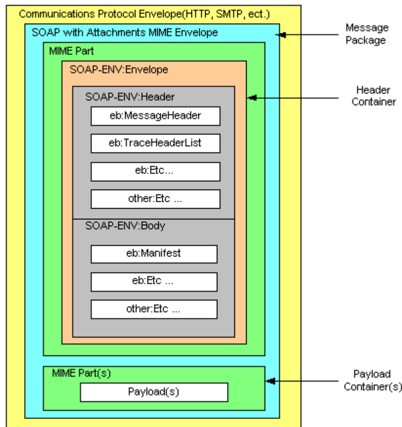
Figure 6-1 ebXML Message Structure
