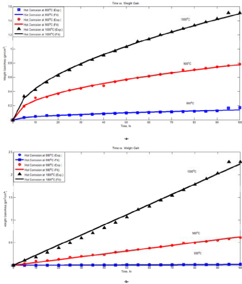
Figure (1 a) weight gain/area vs time plot (parabolic fitted) for Y-doped aluminizing-siliconizing diffusion coated steel-T21 subjected to hot corrosion for 20 cycles at 100 hr for 5 cycle at temperature range (800-1000°C) b) plot of linear-fitted for (weight gain/area) 2 vs time.
