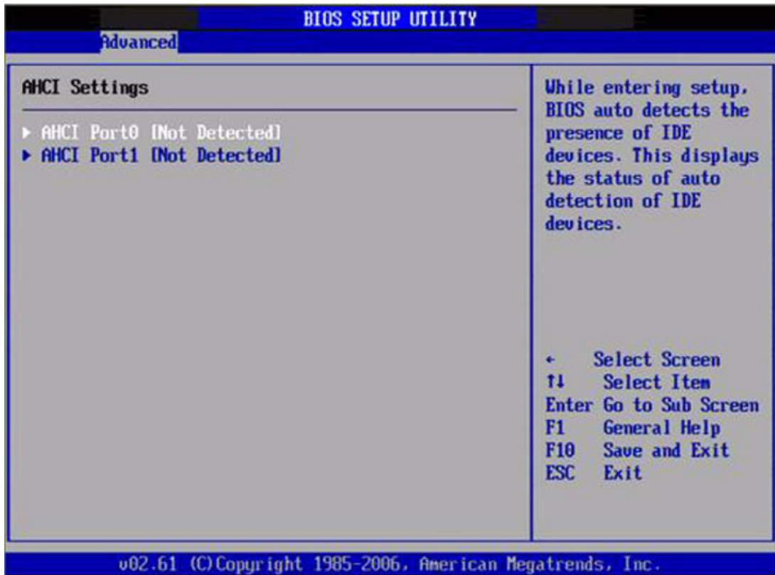
Figure 3.12 AHCI Configuration
