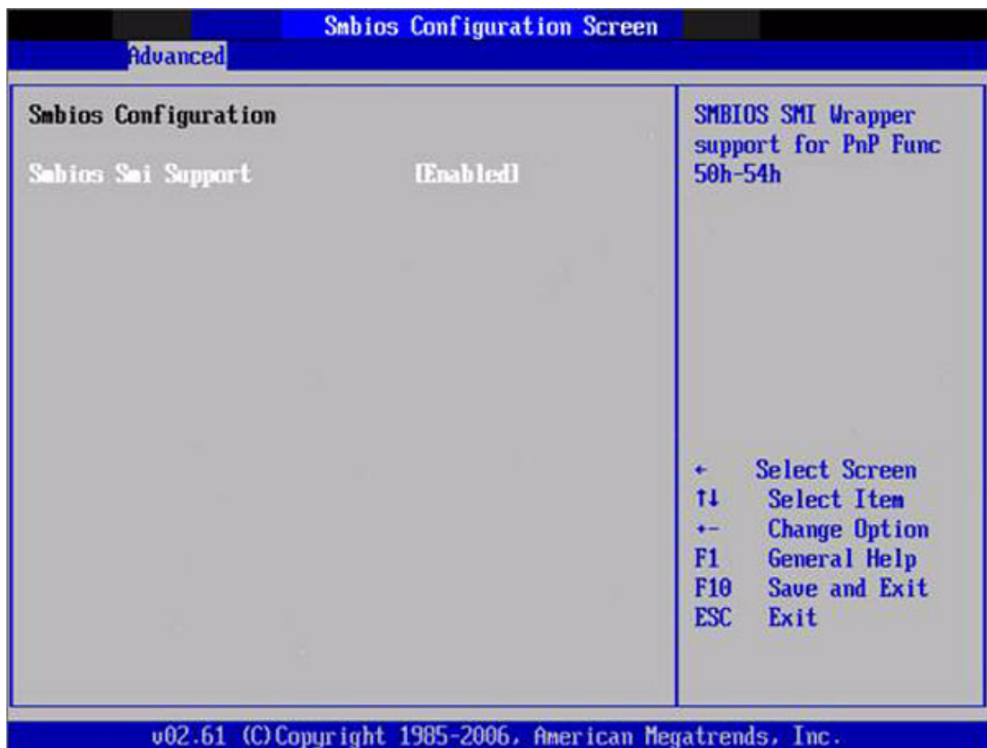
Figure 3.16 Smbios Configuration
