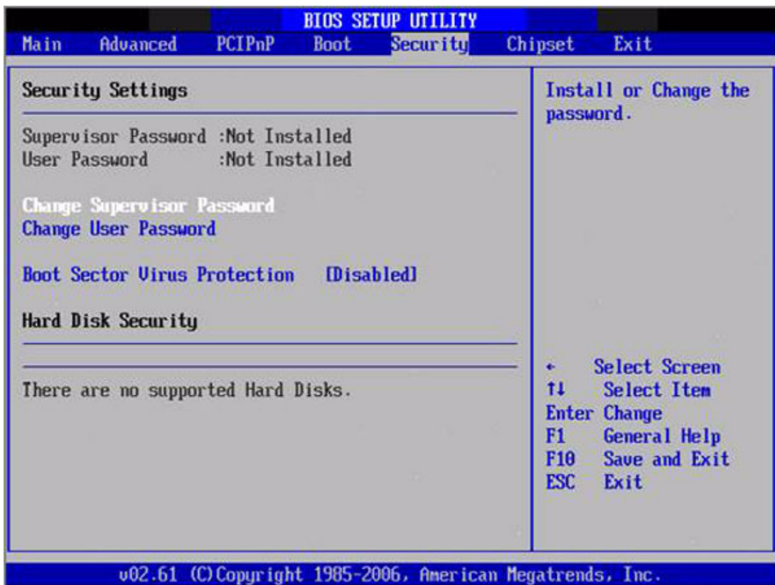
Figure 3.22 Password Configuration
