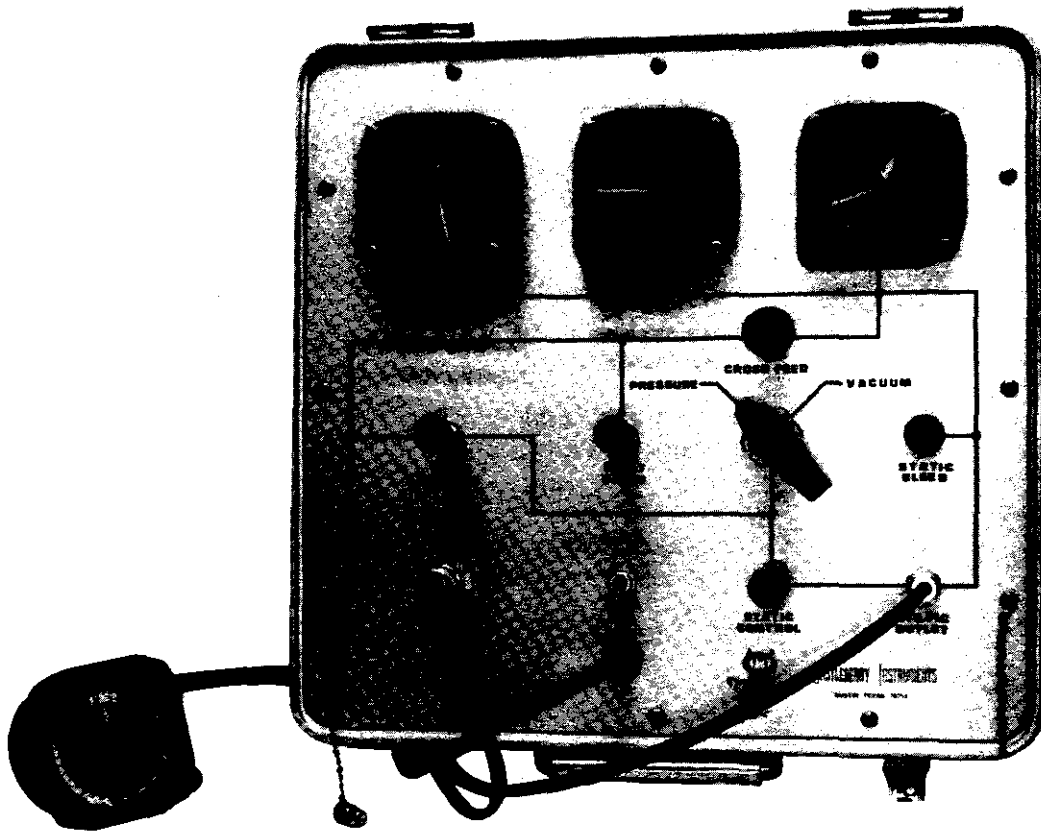
Figure 7.3 Typical Airspeed Indicator Bench Test setup
