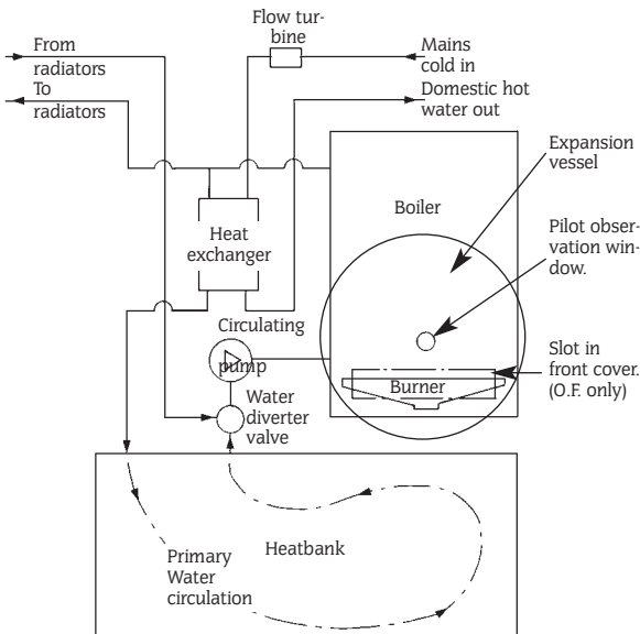
Fig. 1. System Diagram of Highflow 400 Electronic Series.
