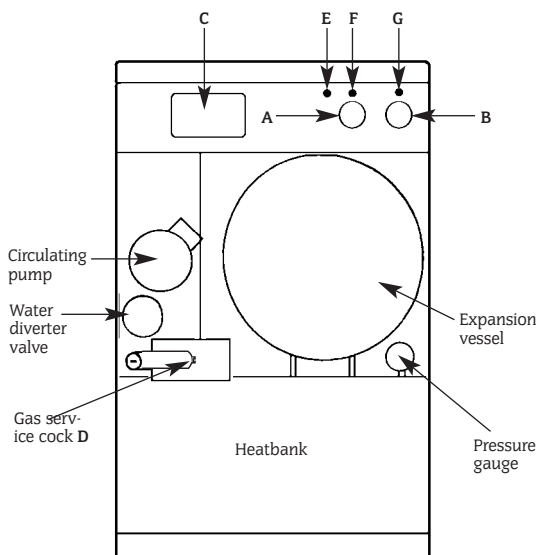
Fig. 3. Appliance with cabinet front cover removed
