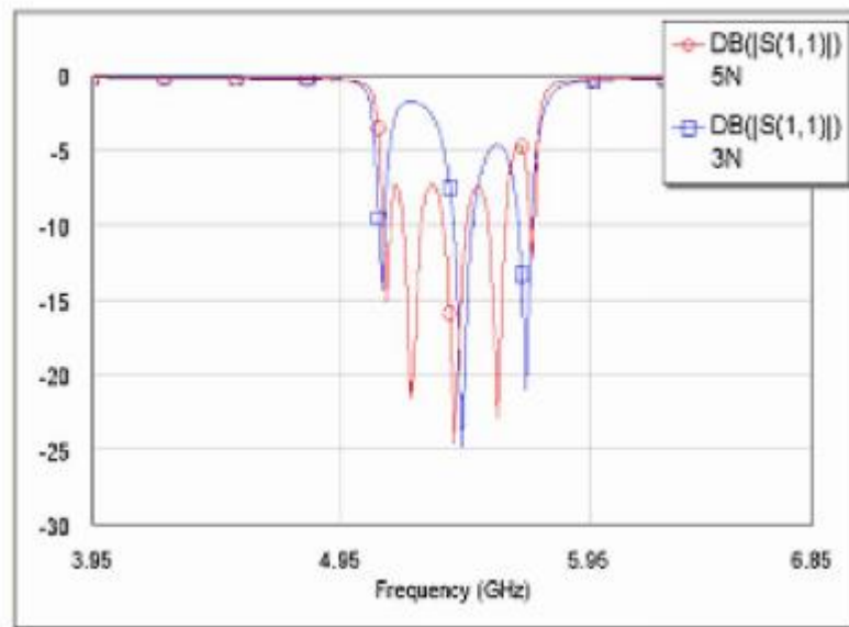
Figure 2.17: S_{11} of third and fifth order filter.
