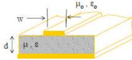
Figure 2.2: Cross section of microstrip.
