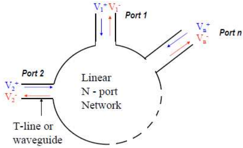
Figure 2.1: Normalized scattering matrix.
