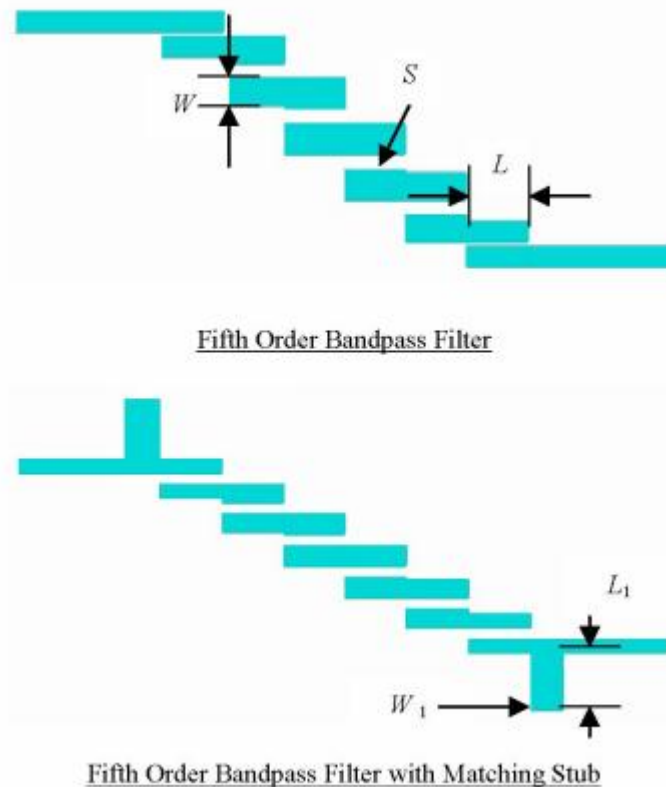
Figure 2.14: Physical layout of bandpass filter.
