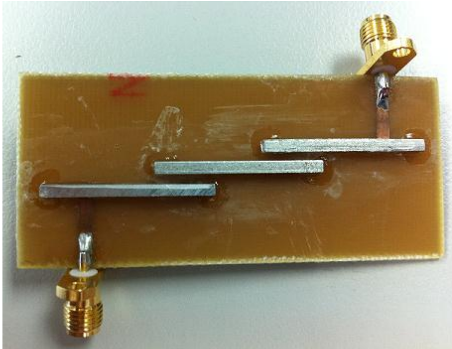
Figure 4.2: Top-down view of the proposed side-coupled block filter.
