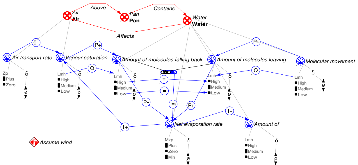
Figure 40: Model fragment 'Mf 3 evaporation assume wind' of the model 'BOKU_LS6 evaporation_advanced'.
