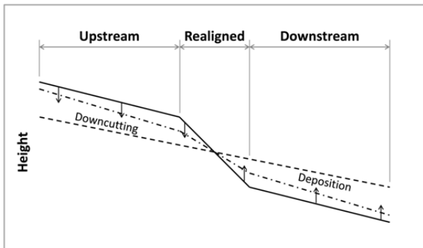
Figure 8: River bed degradation in straightened (realigned) river sections (redrawn from Brookes, 1988).
