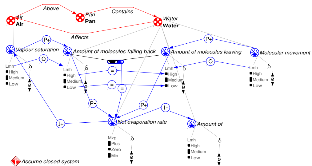
Figure 38: Model fragment 'Mf 1 evaporation closed system of the model' of the model 'BOKU_LS6 evaporation_advanced'.
