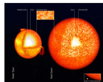
Figure 29: The structure of a solar-like star and a red giant, scale in the lower right corner.
