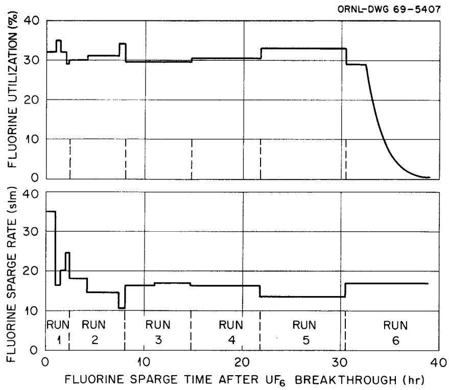
Fig. 17. Fluorine Flow Rate vs Utilization.
