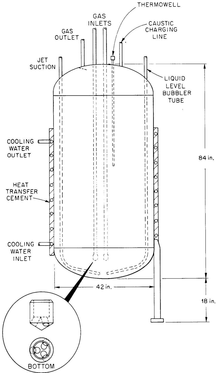
Fig. 7. Caustic Scrubber.
