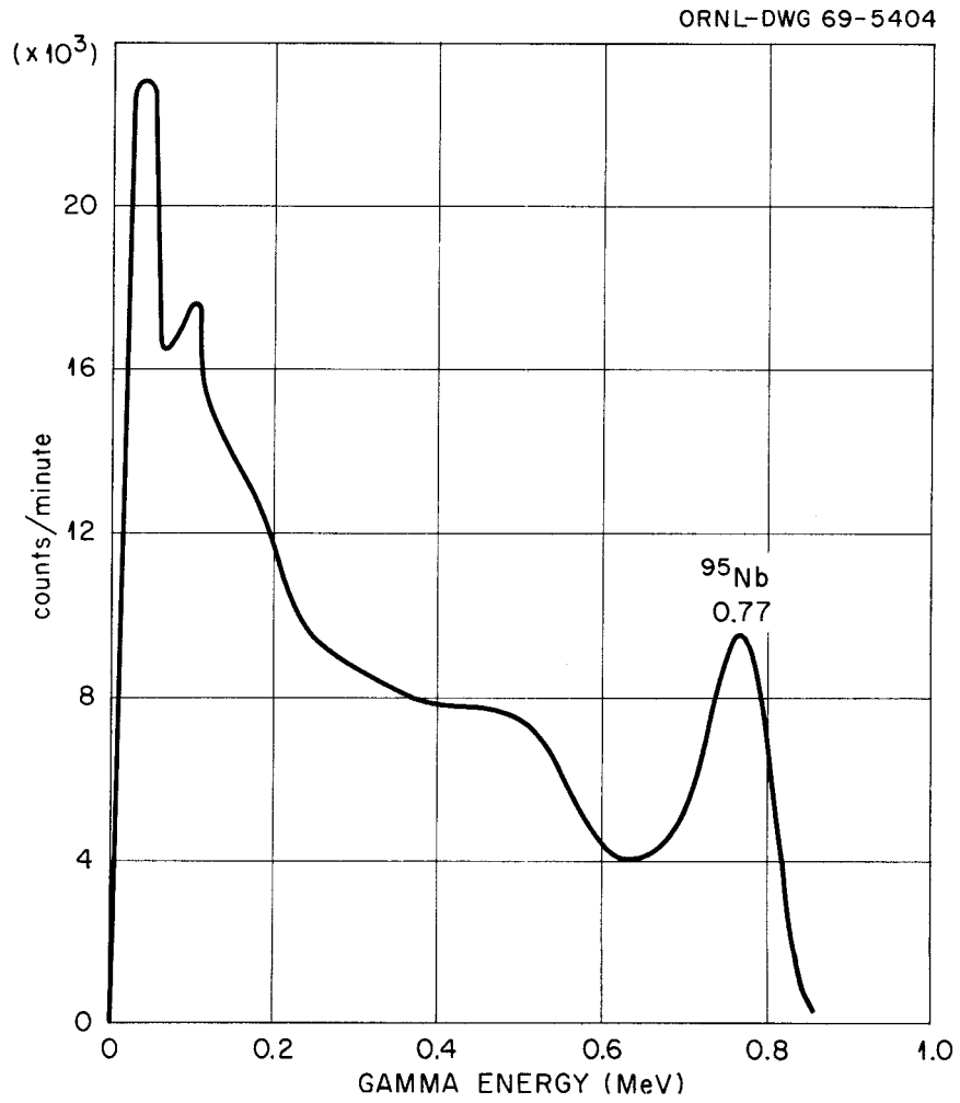
Fig. 22. Gamma Scan of Absorber Cubicle Filter.
