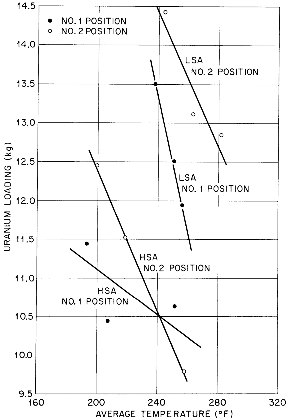
Fig. 23. Comparison of LSA and HSA NaF Loading.
