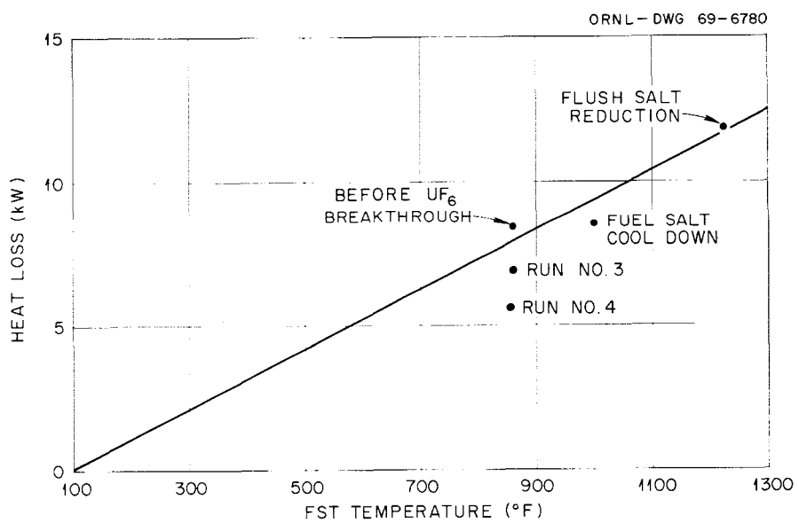
Fig. 5. Fuel Storage Tank Heat Loss.
