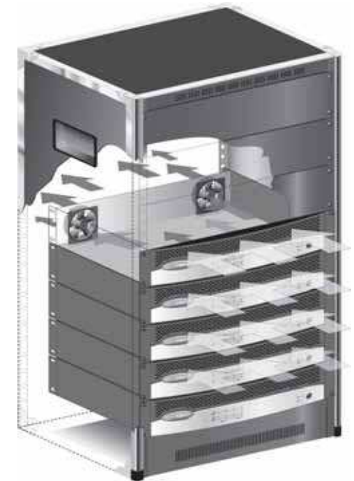
Figure 3.2 Airflow
