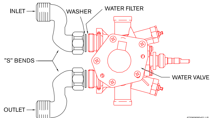
Water valve and S-bends, top view
