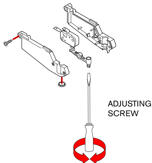
Fig. 13 - Microswitch Adjustment
