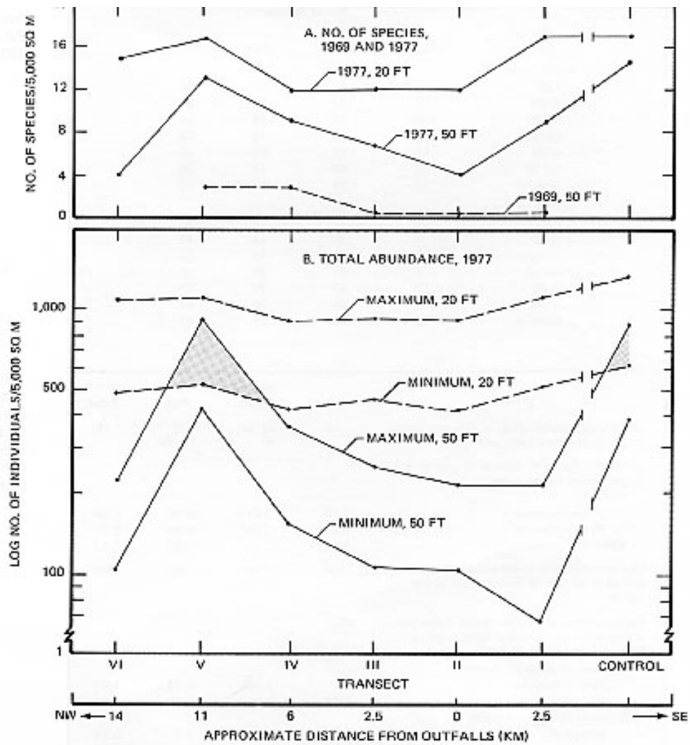
Figure 3. Number of species of algae observed at stations off Palos Verdes and La Jolla in 1969 and 1977 surveys and their cumulative abundance at 20- and 50-ft depths in 1977. Cumulative abundance was calculated twice, assuming all species were present in minimum or maximum abundance. Shaded area represents zone where estimates of abundance at 20 and 50 feet overlap.
