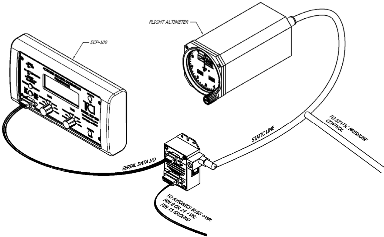
Figure 3 Serial Port Configuration Using the ECP-100
