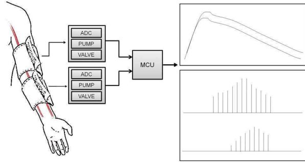
Figure 2. Measurement configuration.
