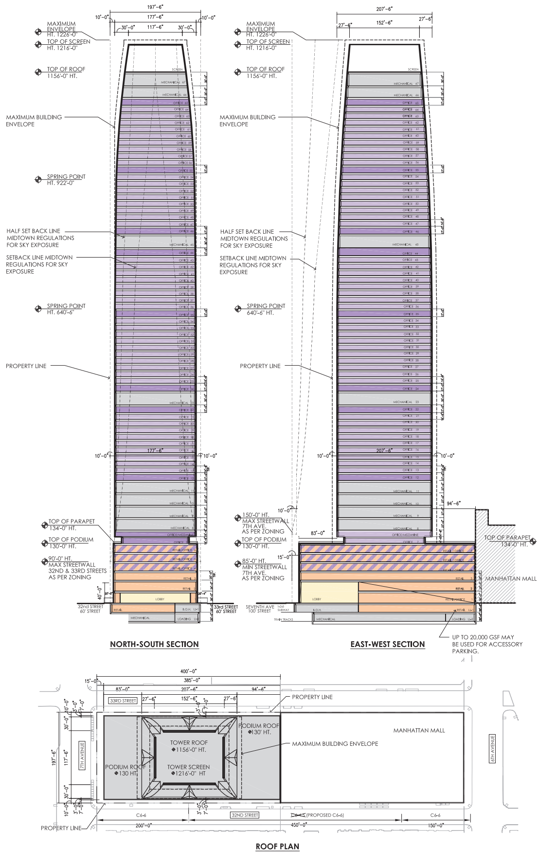
Multi-Tenant Office Scenario Illustrative Building Section Figure 7
