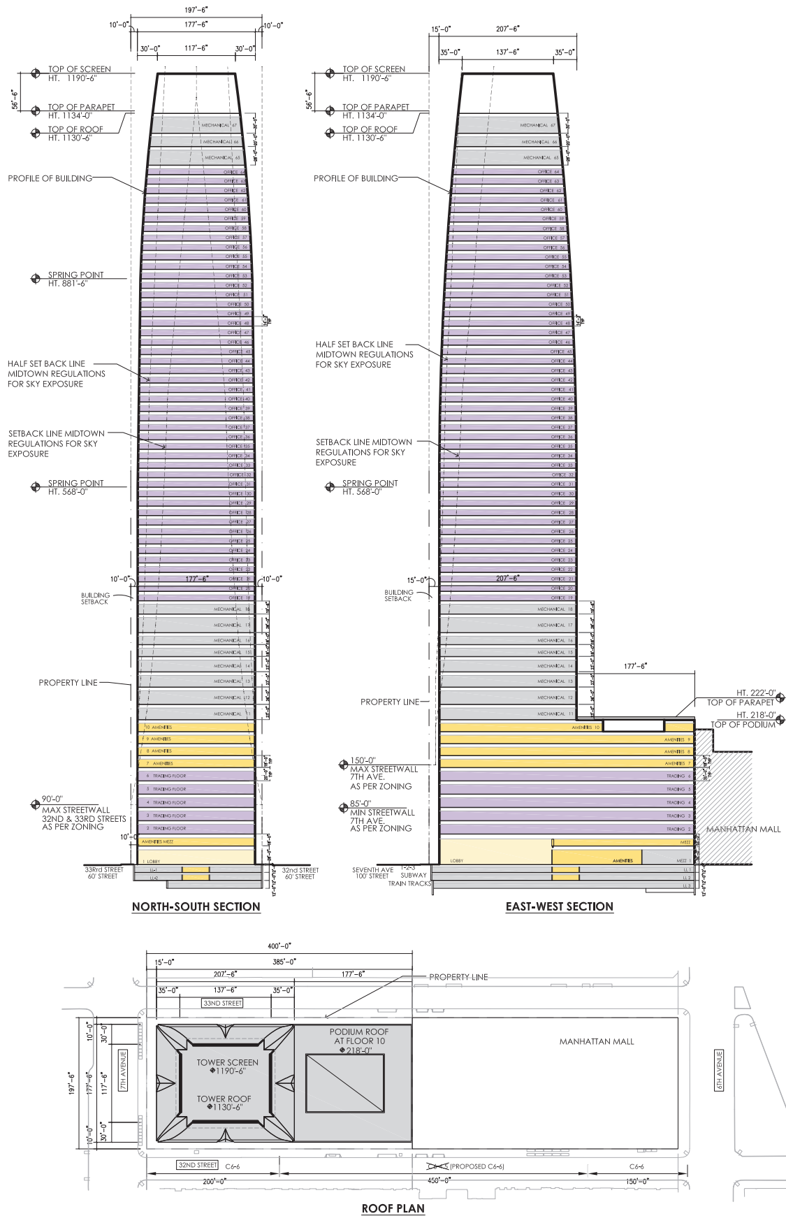
Single-Tenant Office Scenario Illustrative Building Section Figure 5
