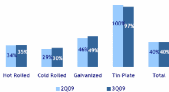
Market Share %
