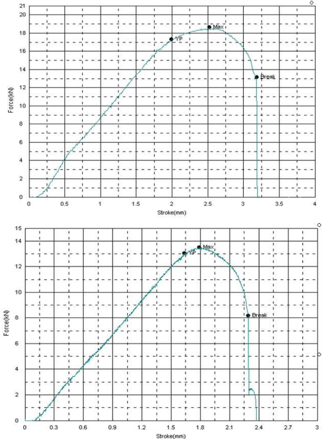
Fig. 4. The Chart of stretching of flat samples of copper (on the right with round cut).
