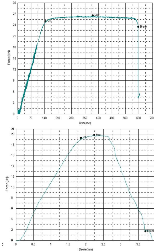
Fig. 3. The charts of stretching of flat samples of brass (on the right with round cut).
