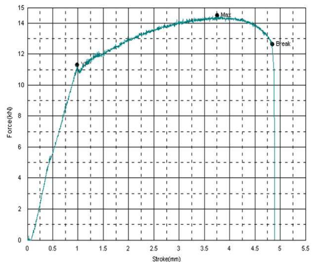
Fig. 5. The chart of stretching of flat steel samples (on the right with round cut).
