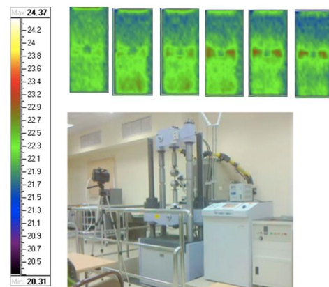
Fig. 2. Tests by the universal equipment of Japanese firm Shimadzu of U1000kHi and the Russian thermovisionary IRTIS 200 (FEFU).
