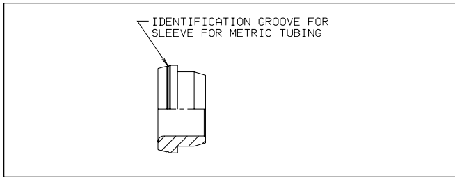
Fig. 14 — Parflange Sleeve for Metric Tubing
