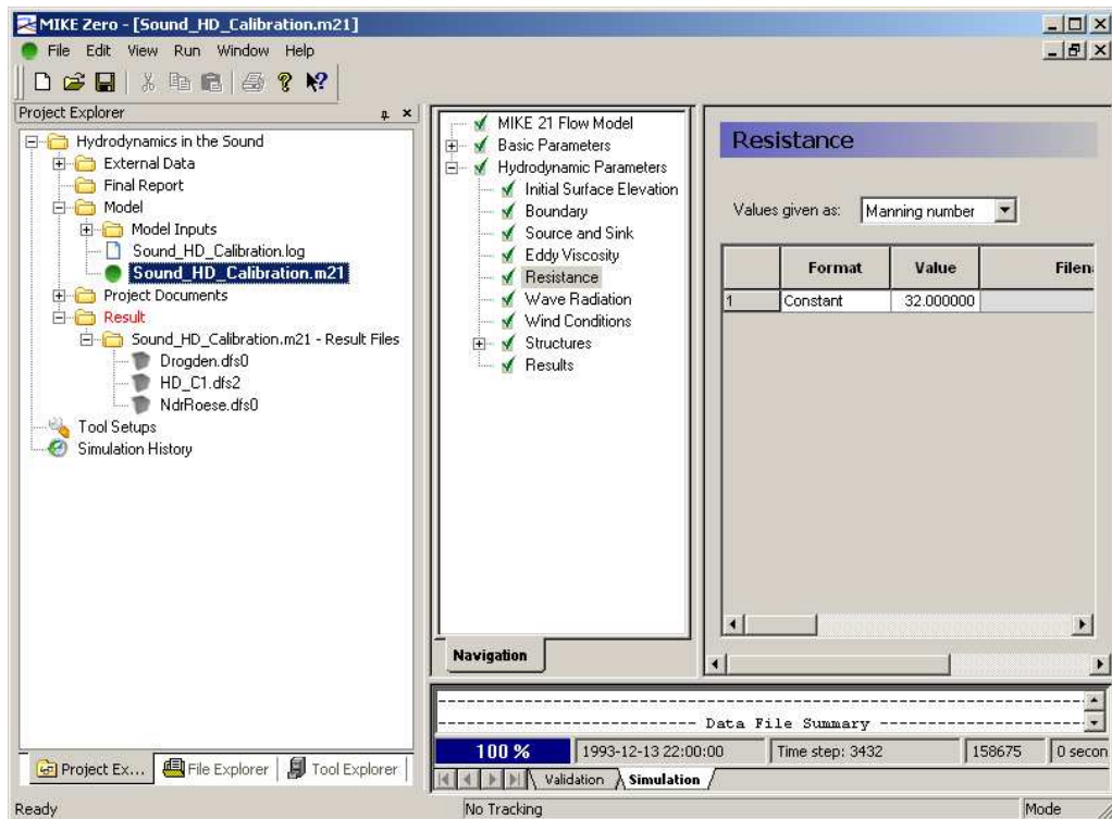
Figure 5.2 Generated output data files shown in the Project Explorer
