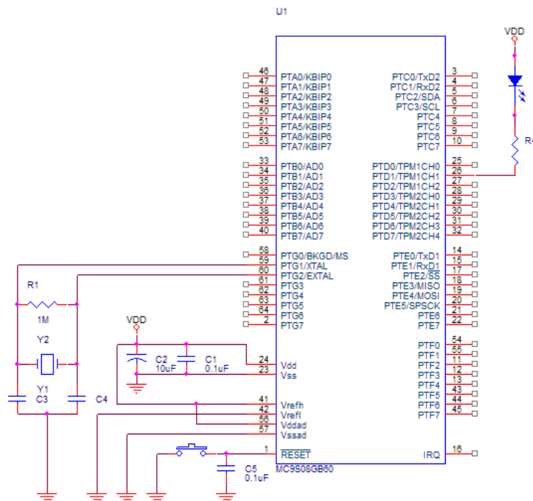
Figure 2. Schematic of Circuit Used in Example 2
