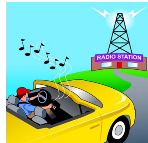
Figure 19.5: You hear music from your car radio when the oscillator in your radio matches the frequency of the oscillator in the transmission tower connected to the radio station.
