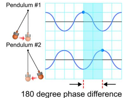
Figure 19.13: The two pendulums are 180 degrees out of phase.
