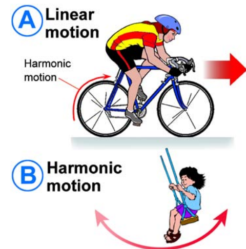
Figure 19.1: (A) Real-life situations such as riding a bicycle can include both linear motion and harmonic motion. (B) A person on a swing is an example of harmonic motion in action.
