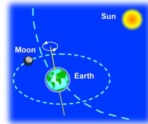
Figure 19.2: The Earth-sun-moon system has many different cycles. The year, month, and day are the result of orbital cycles.
