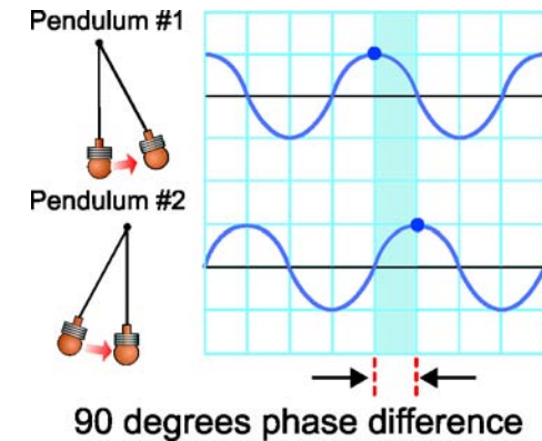
Figure 19.12: The two pendulums are 90 degrees out of phase.
