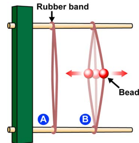
Figure 19.20: A stretched rubber band is a good example of a vibrating string (A). You can modify this simple oscillator by adding a bead to the rubber band (B).
