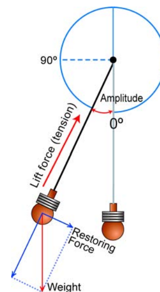
Figure 19.14: Restoring force keeps a pendulum swinging. Restoring force is related to weight and the lift force (or tension) of the string of a pendulum.
