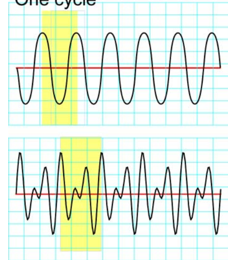
Figure 19.9: The cycle is the part of the graph that repeats over and over. The yellow shading shows one cycle for each of the graphs above.
