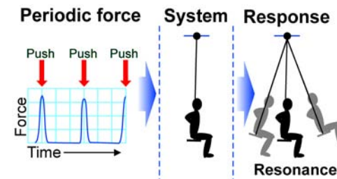
Figure 19.18: When you push someone on a swing, you are using resonance. Small or big pushes at the right time in a swing's motion will make a person swing higher. If the periodic force (the push) is applied at the wrong time, the swing does not swing at all.
