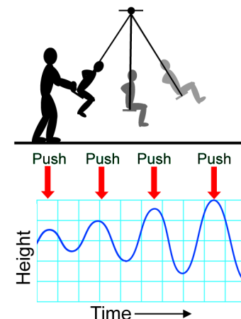
Figure 19.16: Each push of a swing at the right time increases the amplitude (height) of the swing. Each push is a periodic force.
