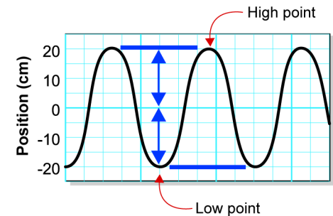
Figure 19.10: The amplitude is one-half the distance between the highest and lowest points on the graph. In this graph of harmonic motion, the amplitude is 20 centimeters.
