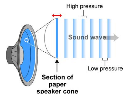
Figure 19.3: As a speaker cone moves back and forth, it pushes and pulls on air, creating oscillating changes in pressure that we can detect with our ears. The dark blue bands in the graphic represent high pressure regions and the white bands represent low pressure regions.
