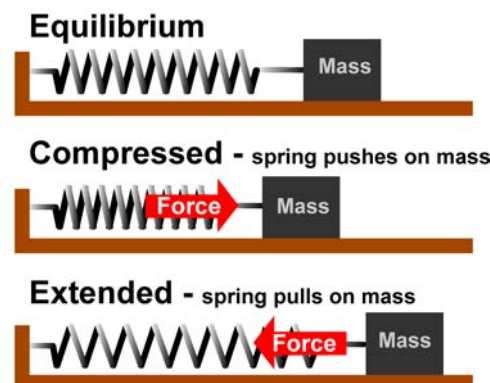
Figure 19.19: A mass on a spring is an oscillating system. When the spring is compressed, it pushes back on the mass to return to equilibrium. When the spring is extended, it pulls the mass back toward equilibrium.
