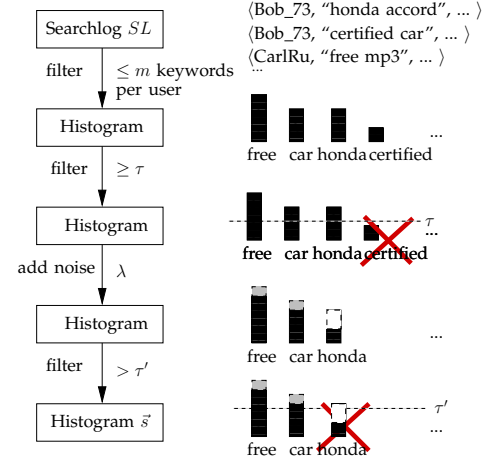
Fig. 1. Privacy-Preserving Algorithm.
