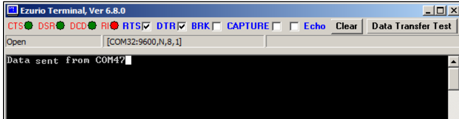
Figure 13: SPP connection
