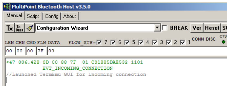
Figure 37: Log activity
