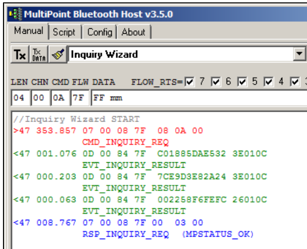
Figure 48: Click Inquire
