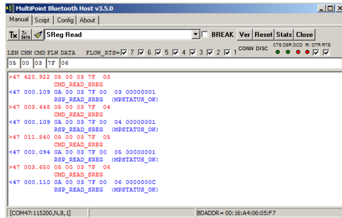
Figure 28: S Registers
