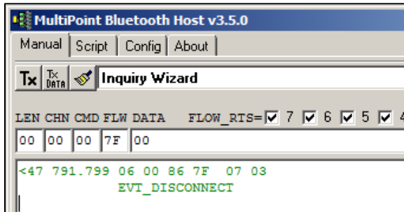
Figure 42: Closed Terminal
