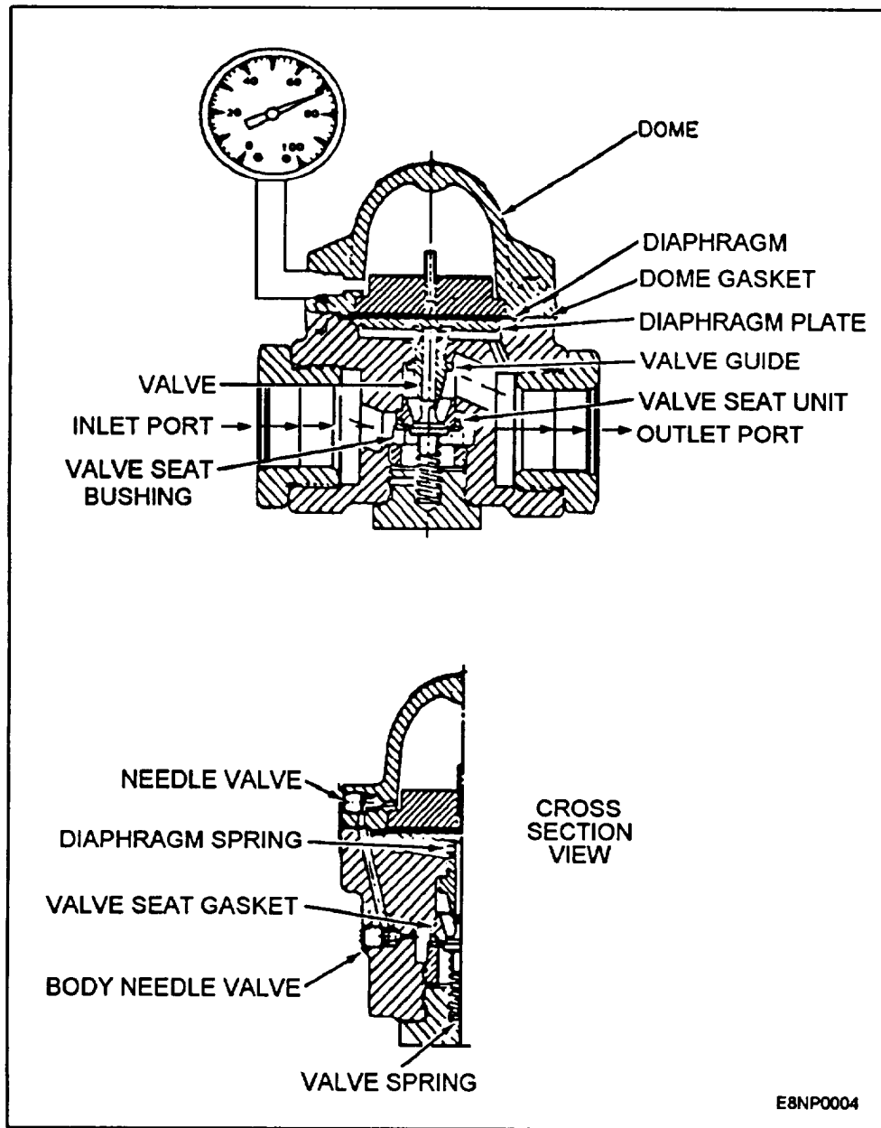
Figure 2-4.-Pressure regulator.
