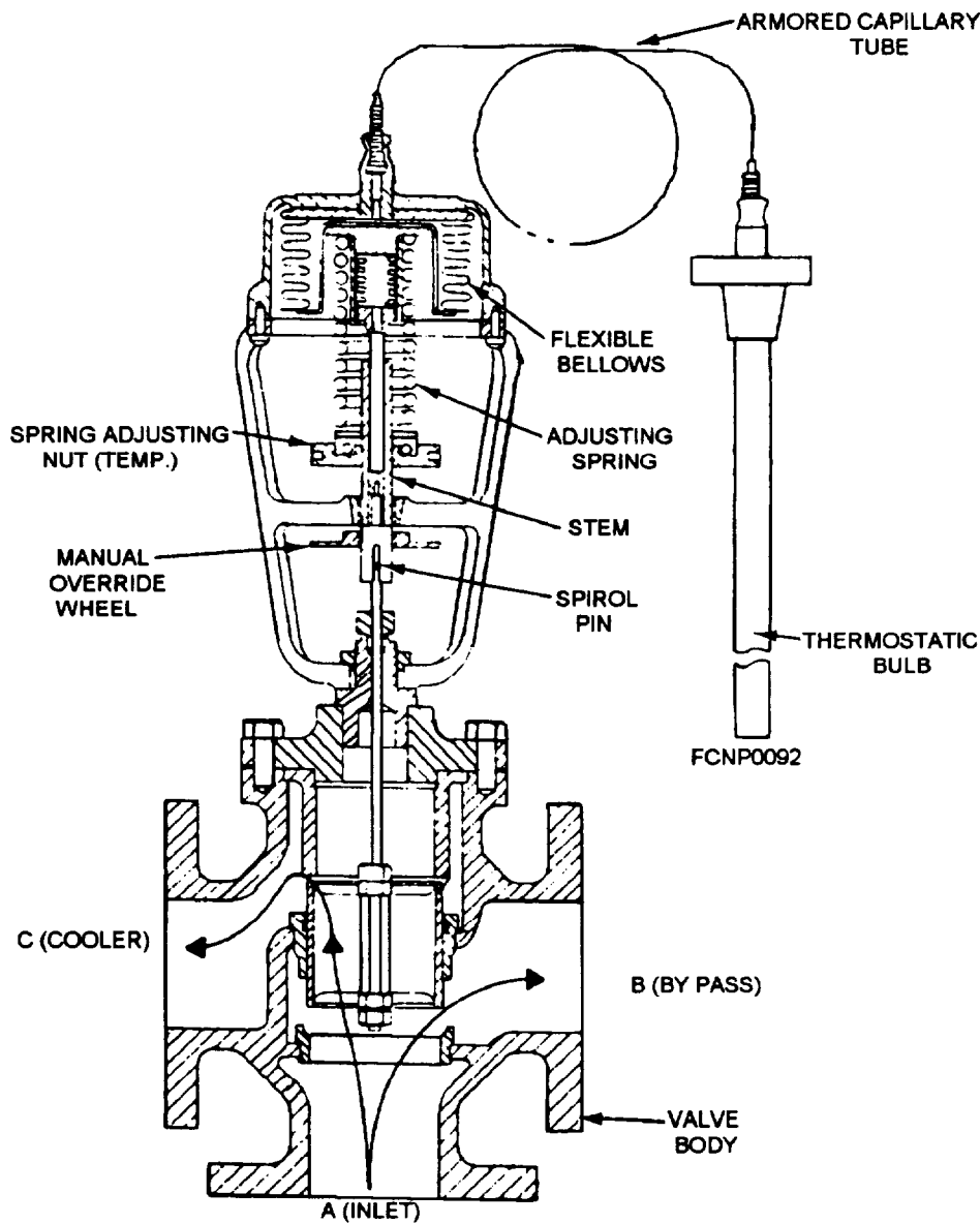
Figure 1-15.—Three-way temperature regulating valve.
