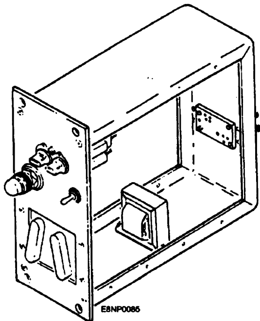
Figure 5-19.-Fuse tester assembly (analog switchboard).
