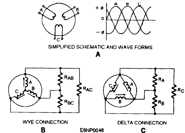
Figure 3-12.—Three-phase ac generator: A. Simplified schematic and wave forms; B. Wye connection; C. Delta connection.
