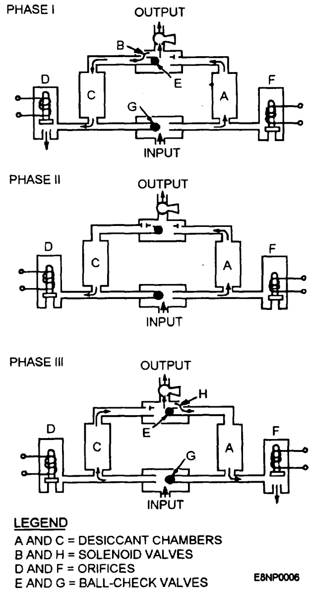
Figure 2-6.—Dehydrator operating cycle.
