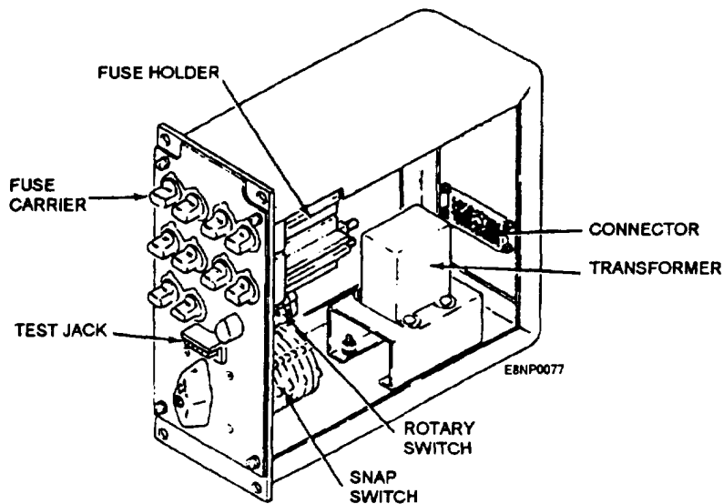
Figure 5-11.—Switch control and potential transformer ACO assembly.
