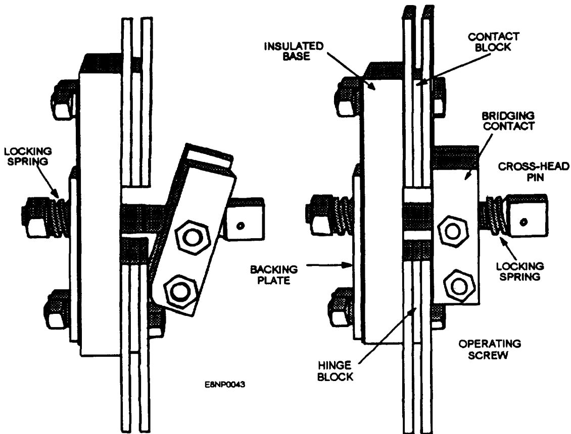
Figure 3-9.-Disconnect links.
