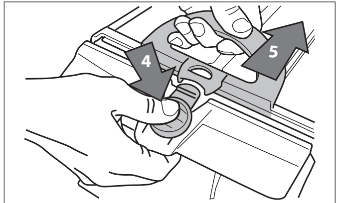
Figure 26. Open Filter Assembly
