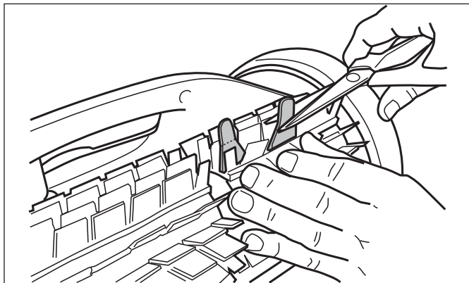
Figure 35. Cut Tabs
