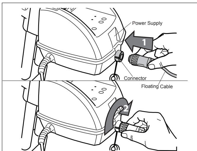
Figure 15. Electrical Connection
