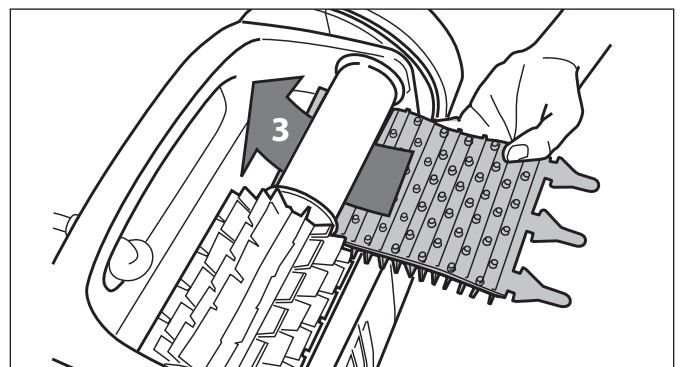
Figure 33. Install the New Brush
