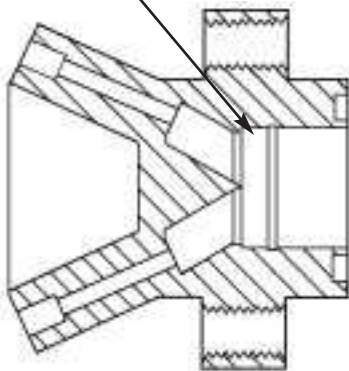
Sporlan Distributor *
