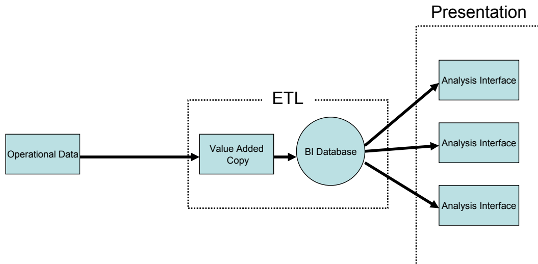
ETL Transforms Operational Data to BI Data
