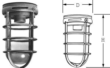
VK1GC Ceiling Unit with Cast Guard and Glass Globe
