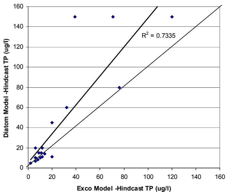
Figure 7 Scatterplot of Hindcast TP concentrations produced by the export coefficient models versus the diatom models for selected test lakes in England, Wales and Scotland.
