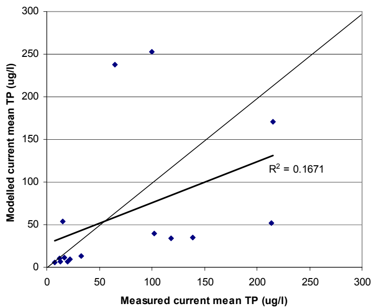
Figure 6b Scatterplot of measured current mean TP concentrations versus those modelled by the eutrophication protocol using people and land cover only for selected test lakes in England and Wales. The linear regression line, the R^2 value and the 1:1 line are shown.
