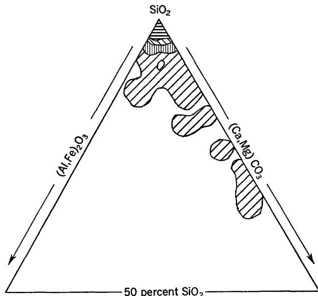
NODULAR CHERT IN CARBONATE ROCK (57 analyses)
