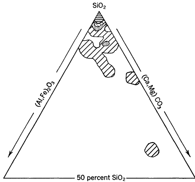
SPICULAR CHERT (24 analyses)
