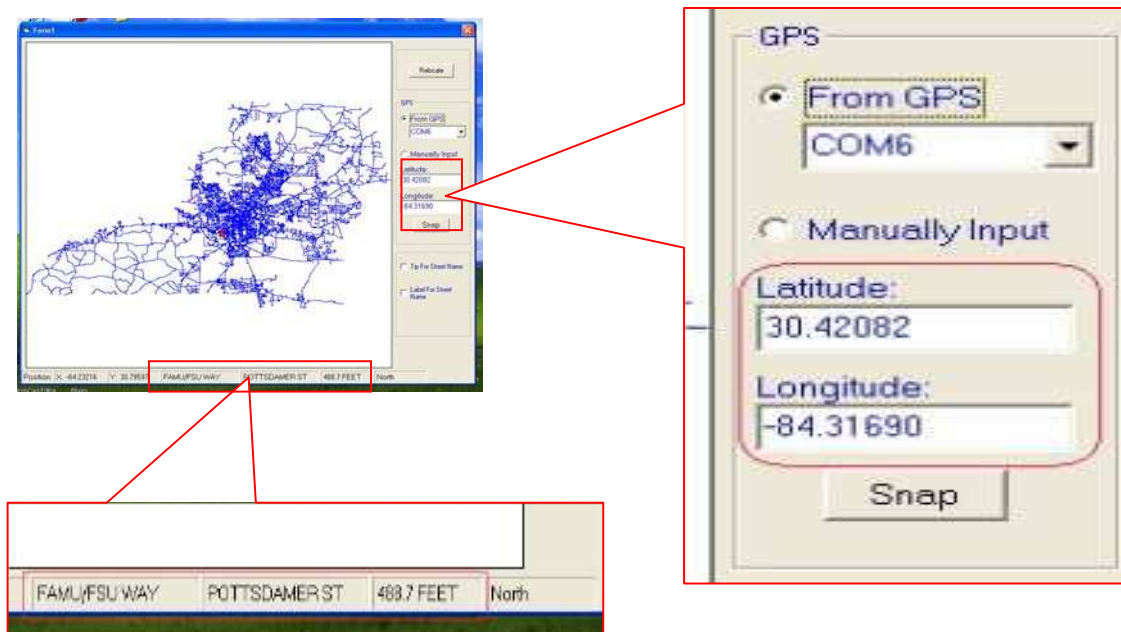
Figure 4: GPS/GIS integration
