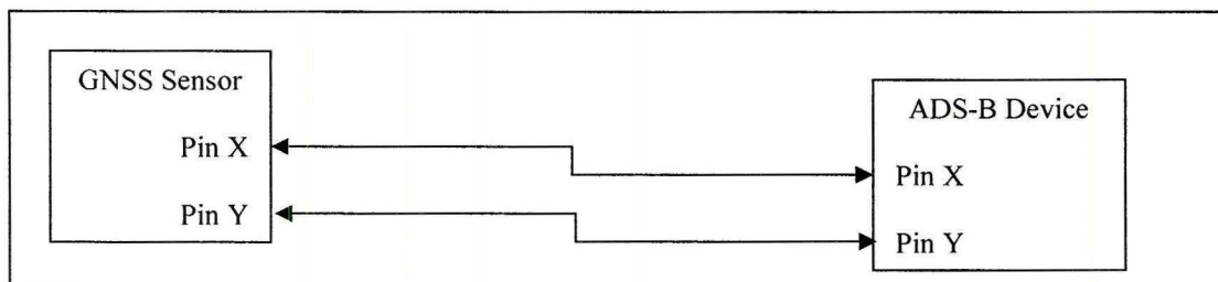
Figure 1: ADS-B/GNSS Sensor Installation Wiring
