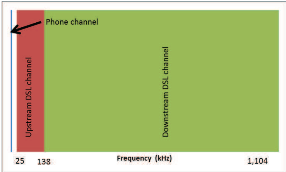
Figure 16.4: Phone and DSL signal frequencies
