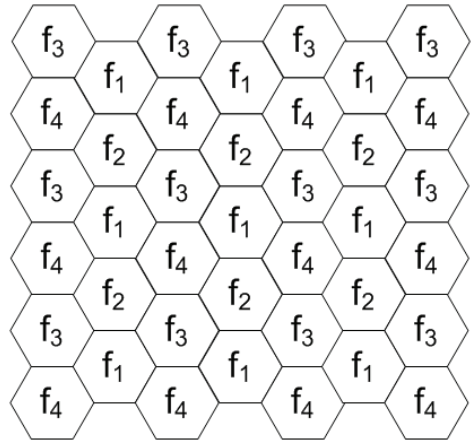
Figure 16.8: Cell phone frequency reuse pattern example
