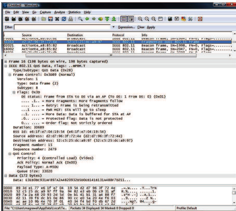
Figure 15.4: Header fields in a captured wireless frame
