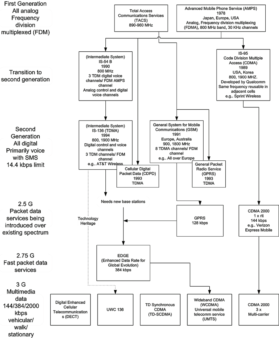
Figure 16.6: Cell phone technology evolution
