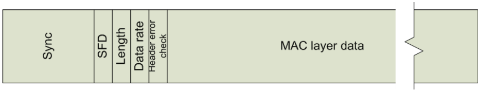
Figure 15.5: Wireless LAN physical layer header
