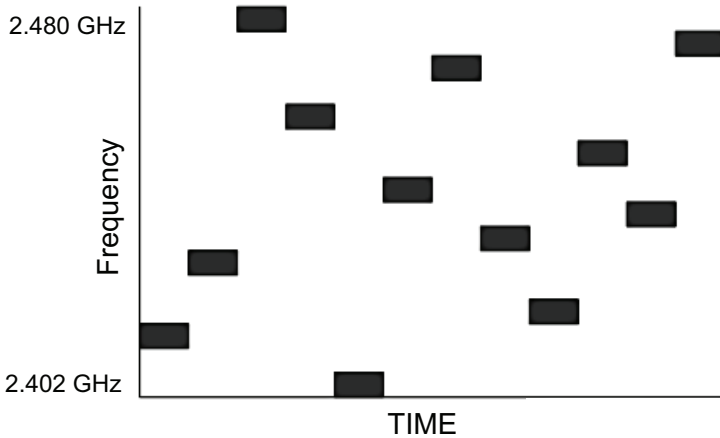
Figure 15.6: Bluetooth frequency-hopping transmission
