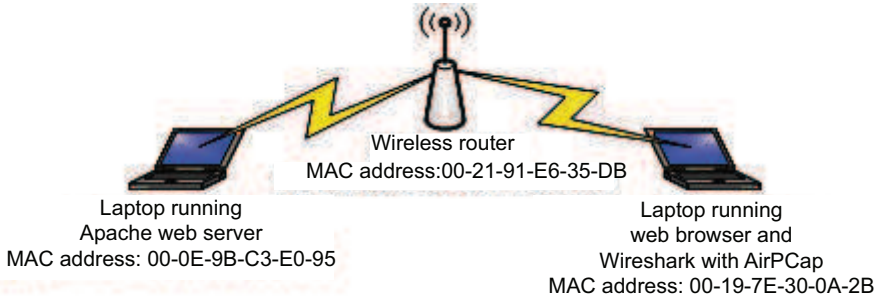
Figure 15.10: AirPCap capture topology
