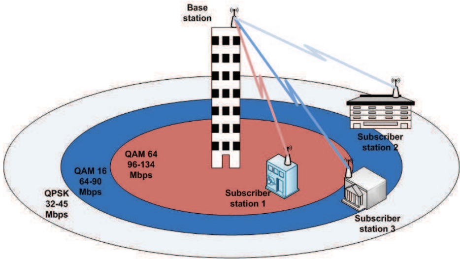
Figure 15.8: WiMAX data rates
