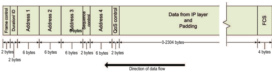
Figure 15.3: 802.11 frame format
