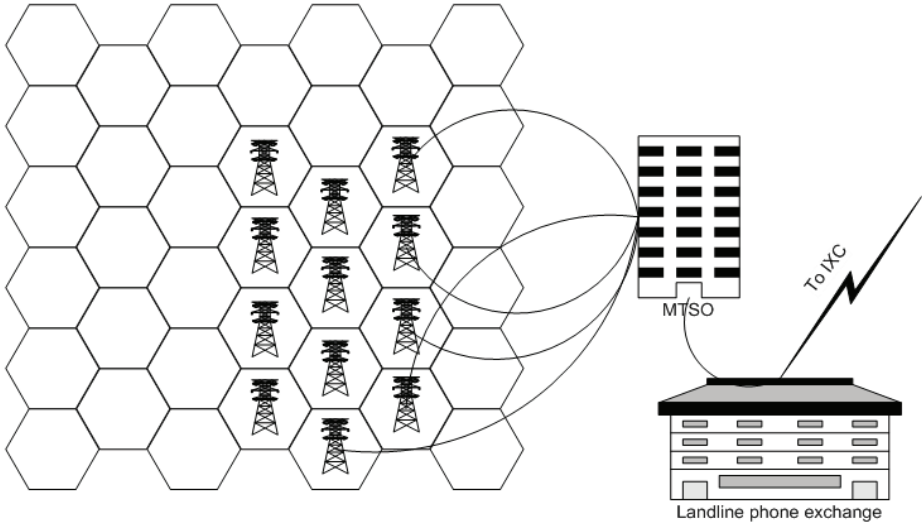
Figure 16.7: Cell phone system architecture
