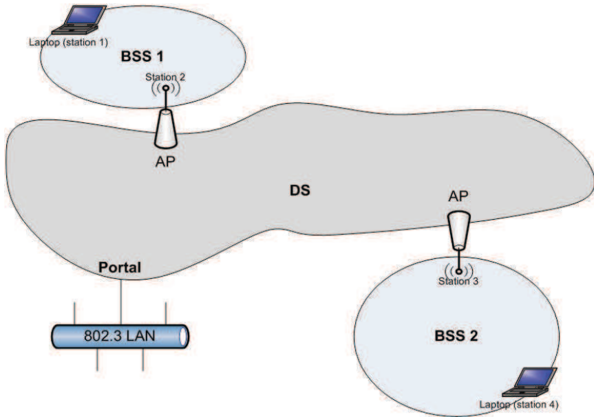
Figure 15.2: Structure of a campus-wide wireless LAN
