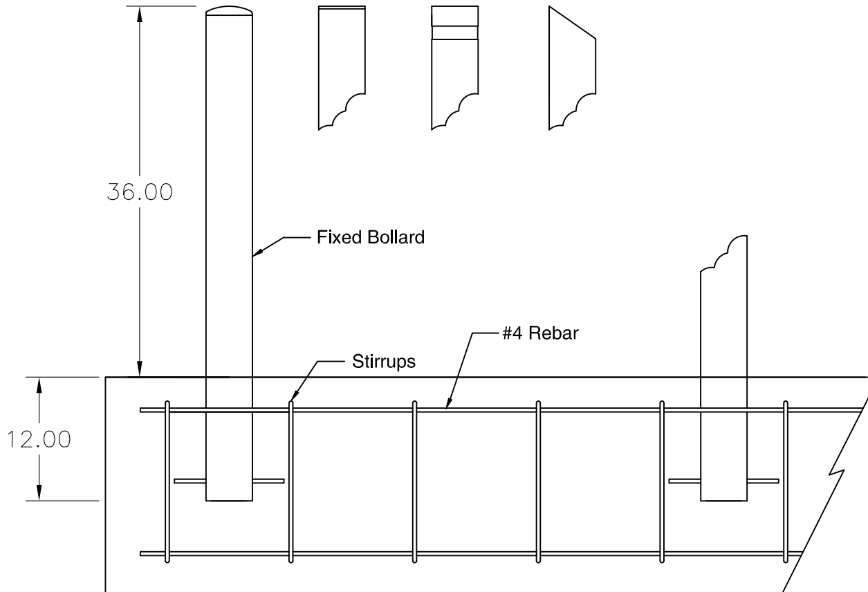
ELEVATION VIEW - FOUNDATION
