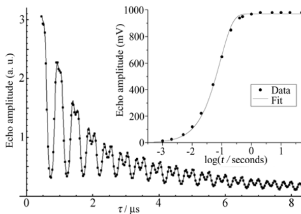
FIGURE 1. Two-pulse ESEEM data from the low field hyperfine line of sample 1. Dots show every fourth data point. The line shows the best fit of the two population model E(\tau) ; see also table 1. Inset: Fit of V(t) to recovery time data from the middle hyperfine line of sample 2.
