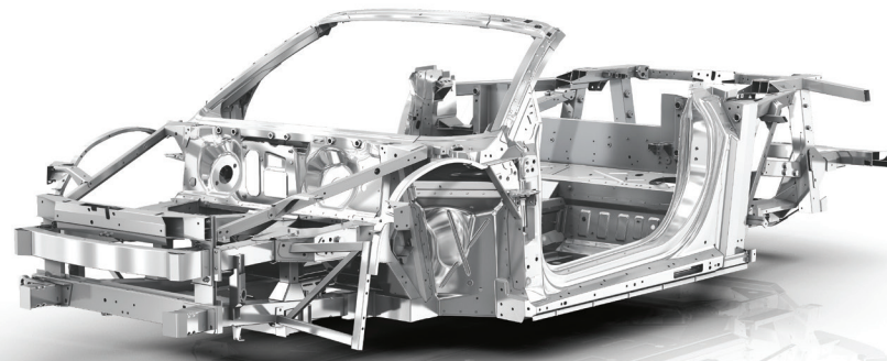
Audi R8 ASF® aluminum construction
