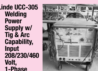
Linde UCC-305 Welding Power Supply w/ Tig & Arc Capability, Input 208/230/460 Volt, 1-Phase Output 100 Amps, AC/DC
