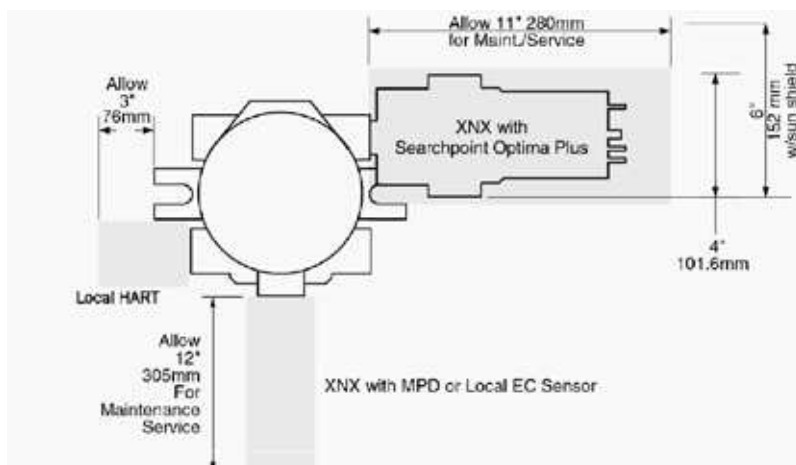
Figure 2. XNX Universal Transmitter mounting dimensions and clearances
