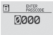
Figure 37. Passcode screen
