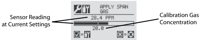
Figure 46. Span Calibration screen
